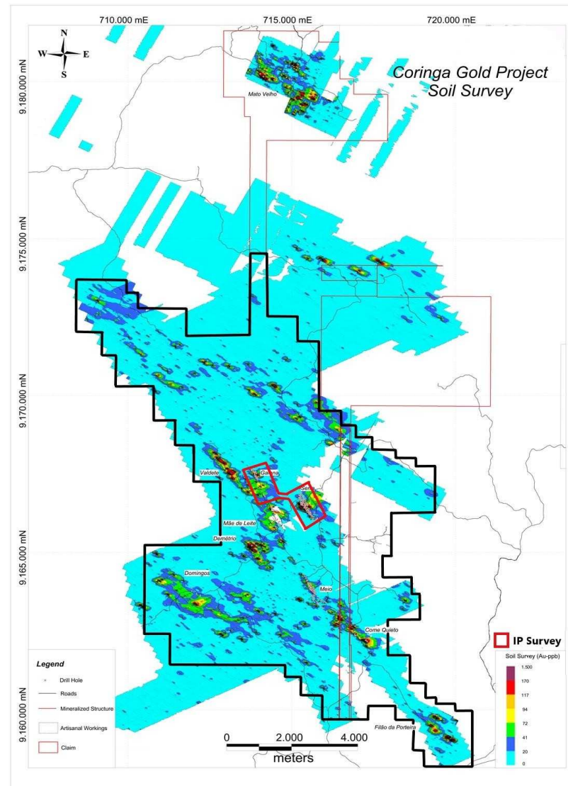
Soil Survey
