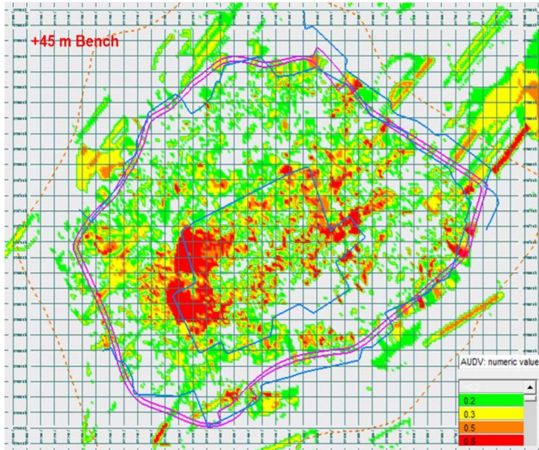
+45 m Bench gold grade distribution
