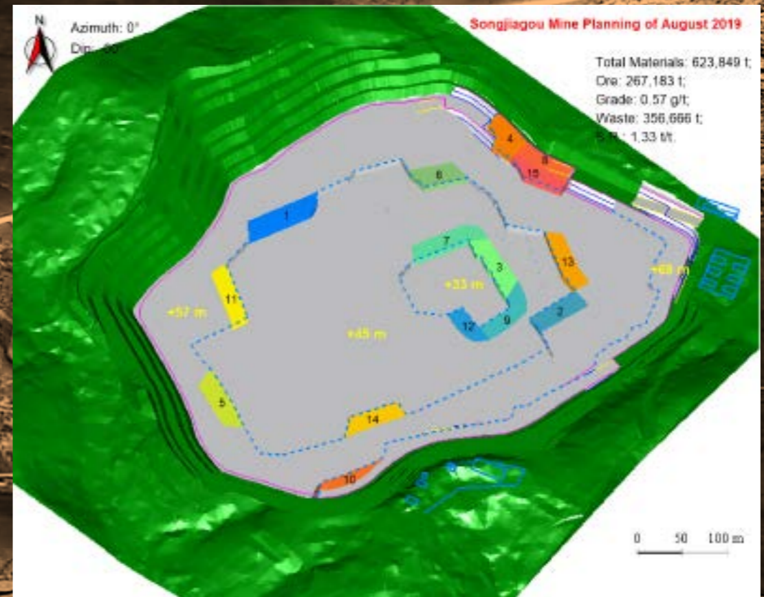
August 2019 Monthly Mine Plan
