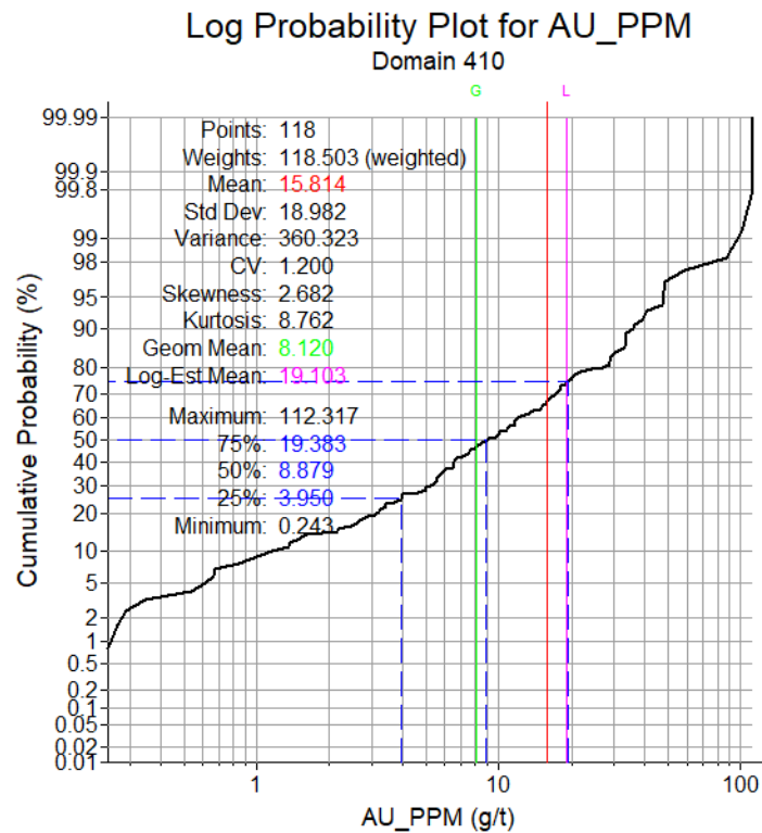
Figure 14.2 Log Probability Plot of the EG Vein, WKP
