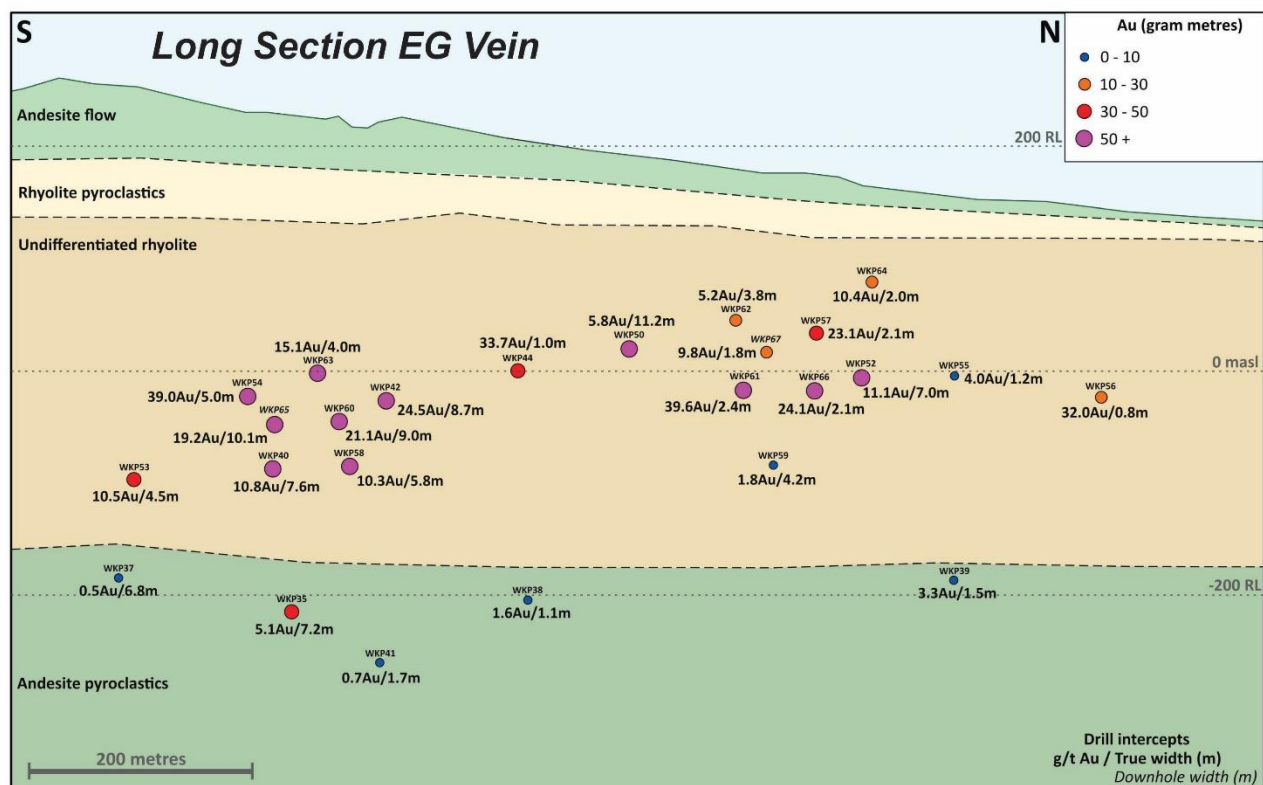
Figure 7.4: Simplified Cross and Long Sections along the EG Vein at WKP.
