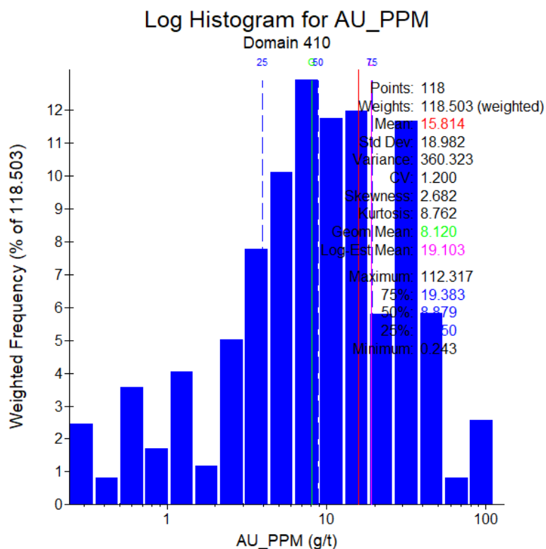
Figure 14.3 Log Histogram Plot of the EG Vein, WKP
