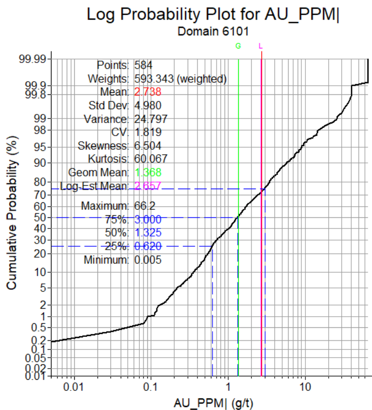
Figure 14.4 Log probability Plot for the 6101 domain, Gladstone
